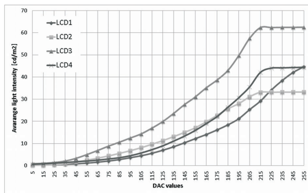
Fig. 3. LCD monitors' gamma characteristics in case of red colour stimulus.
