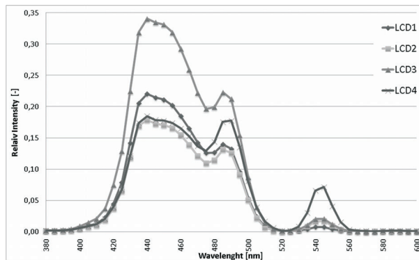
Fig. 2. LCD monitors' spectral output distributions in case of blue colour stimulus.
